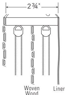
STANDARD TWIN SHADE Controls Same Side (shown) or Opposite Sides
