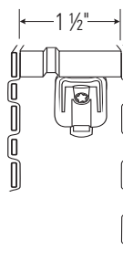
CORDLESS HEAD RAIL • Standard Shades • Waterfall Shades
